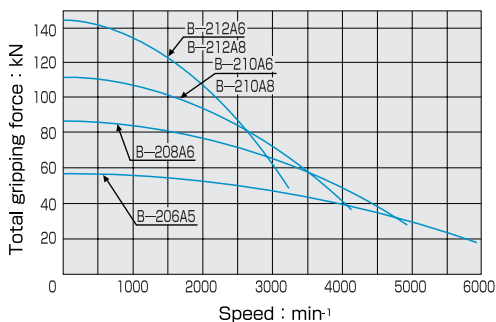
Gripping Characteristic Graphs B-200A
